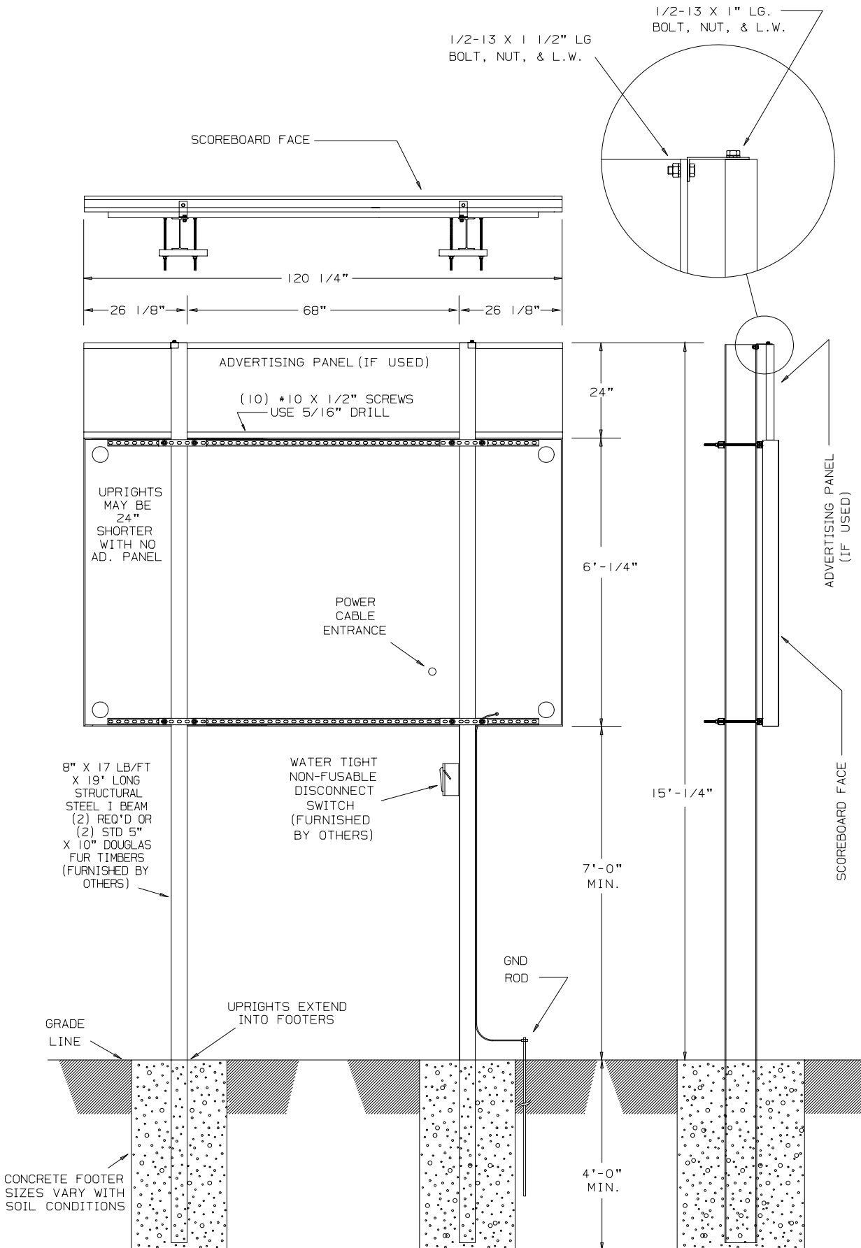
INSTALLATION DRAWING
